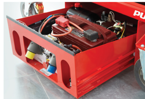
Slide-out service tray for easy maintenance
